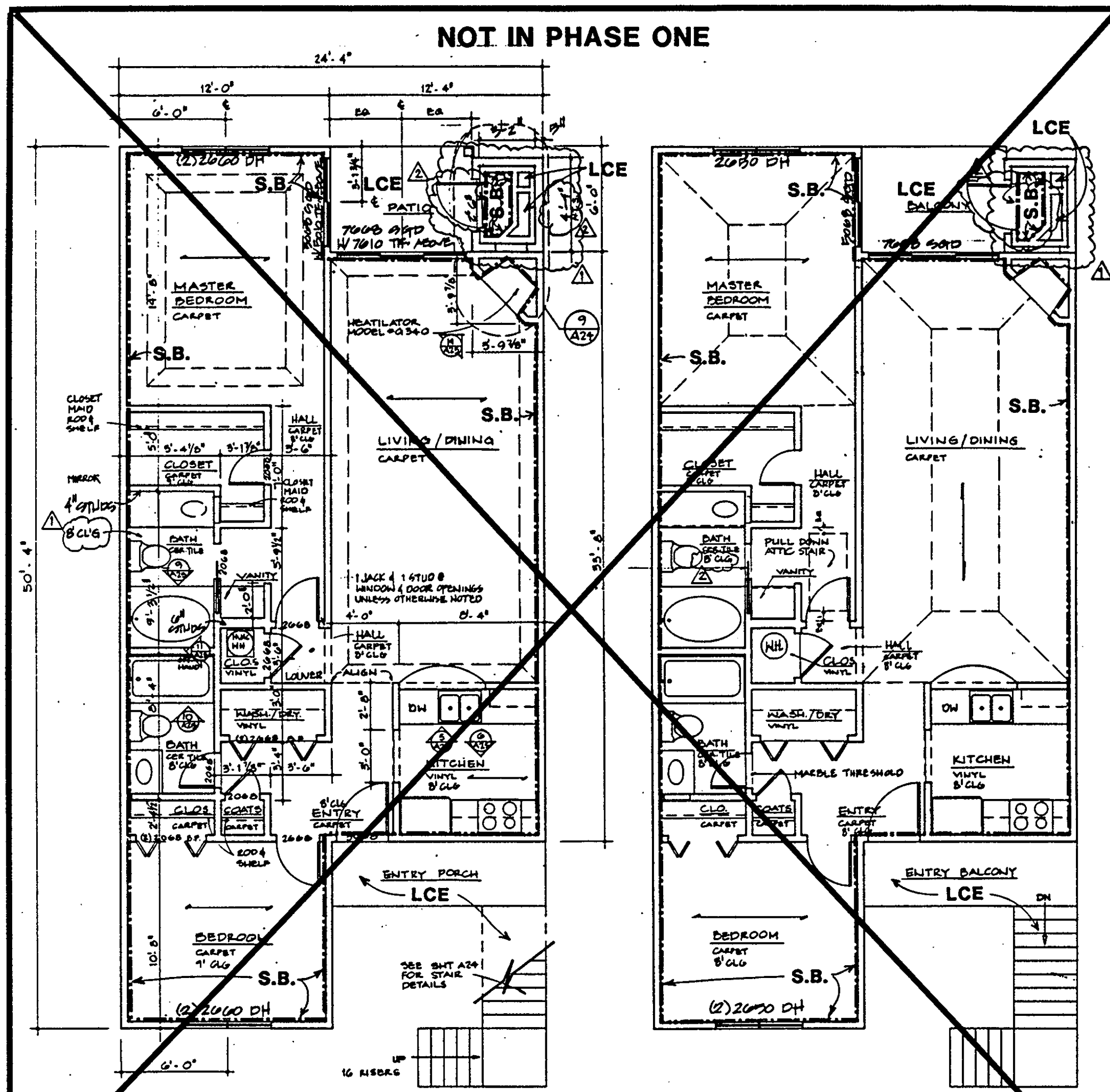
FIRST FLR. PLAN - UNIT 'C'
