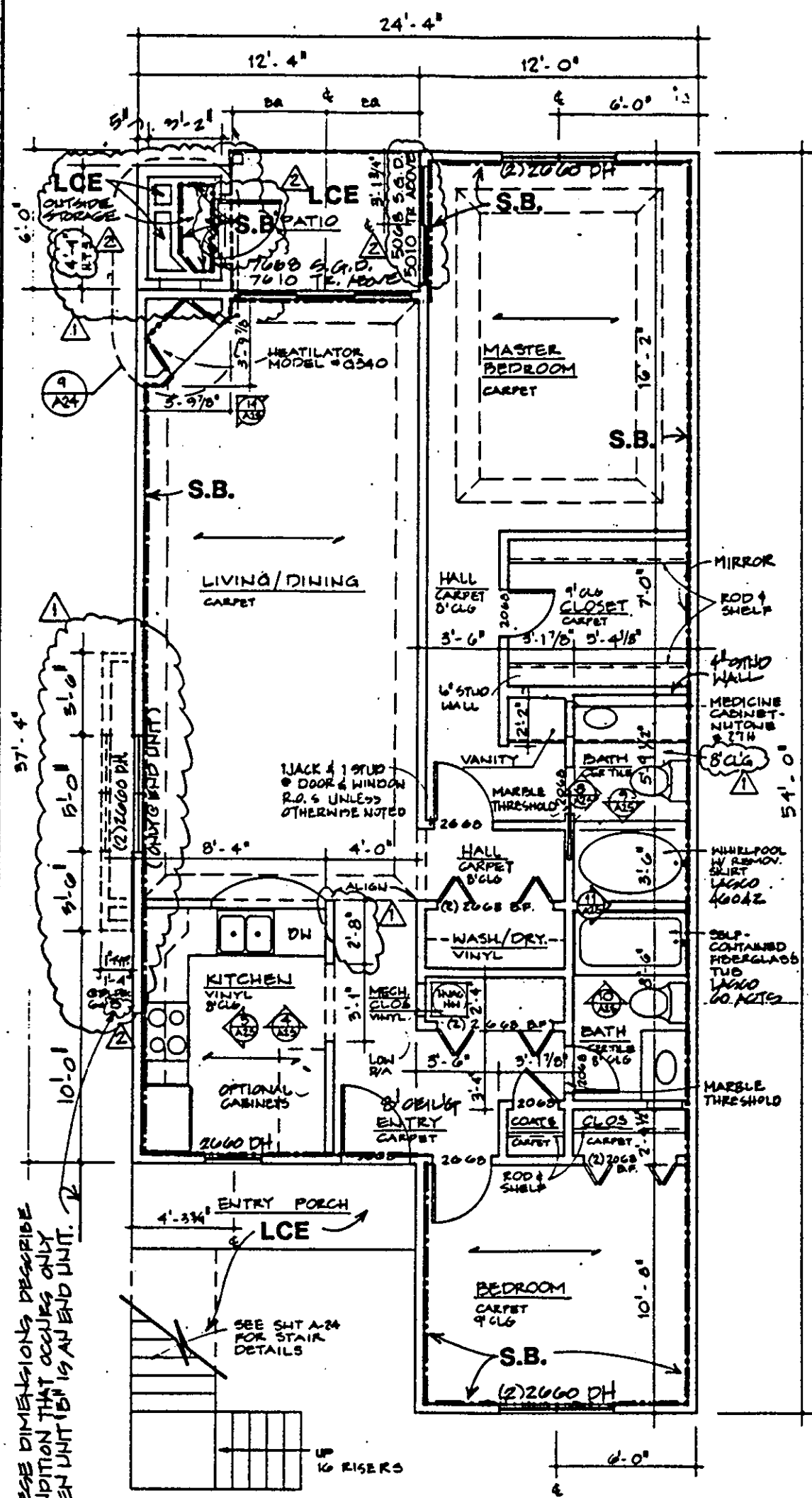
FIRST FLR. PLAN - UNIT 'B'
