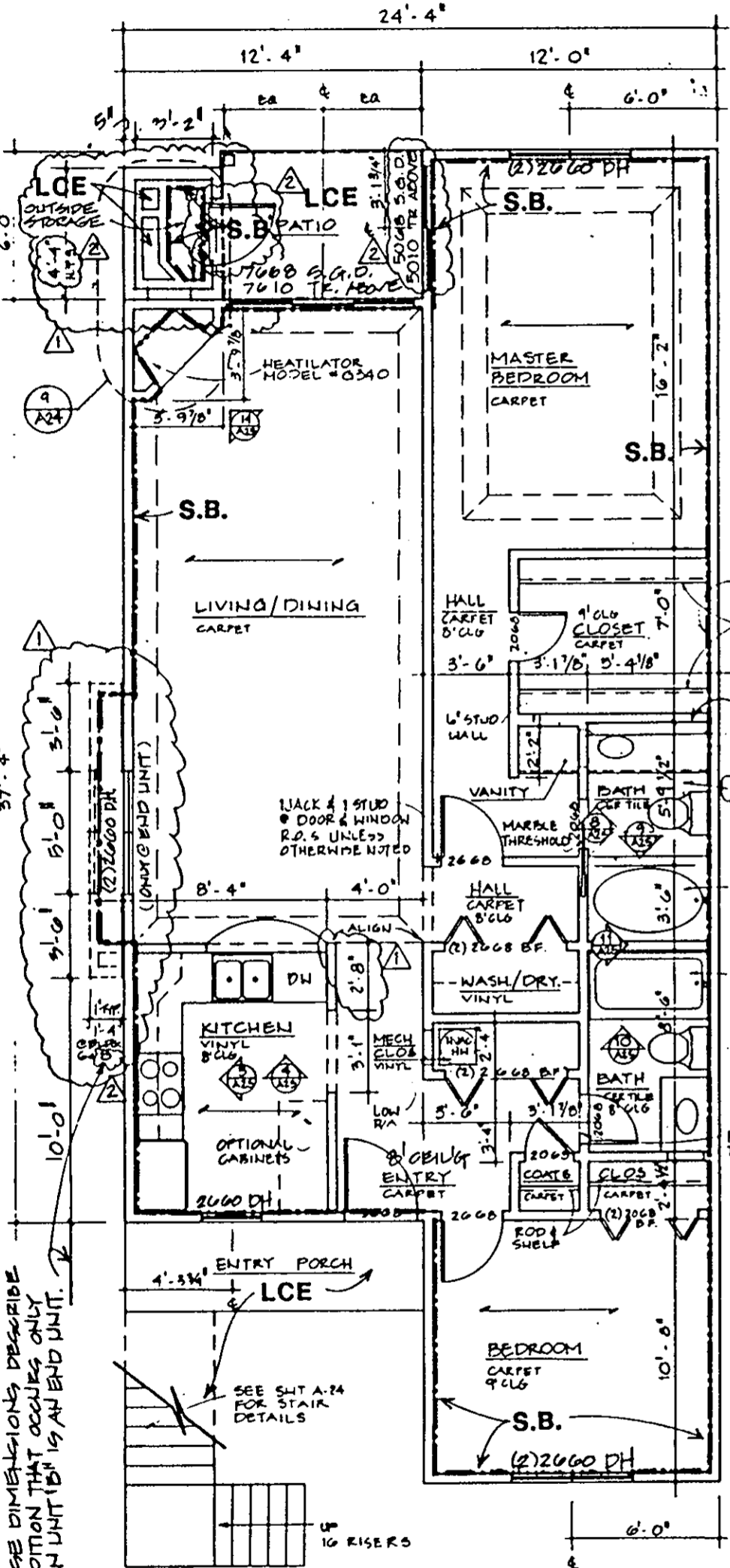
FIRST FLR. PLAN - UNIT "B"
