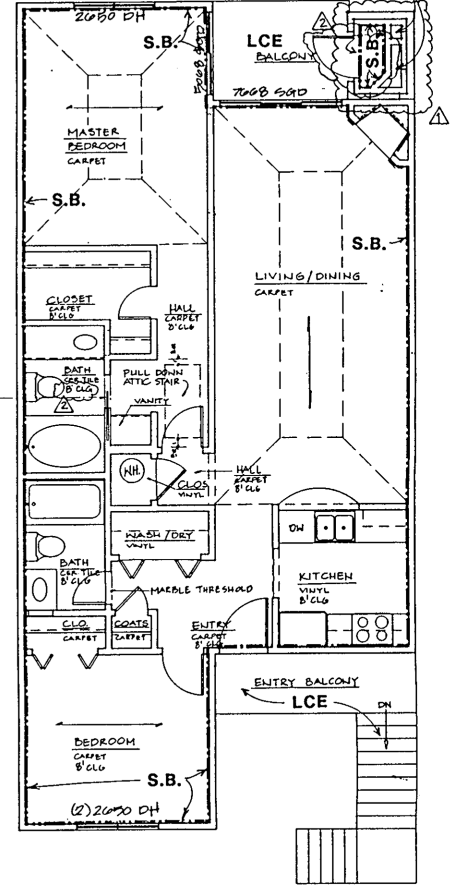
SECOND FLR. PLAN - UNIT "C"
