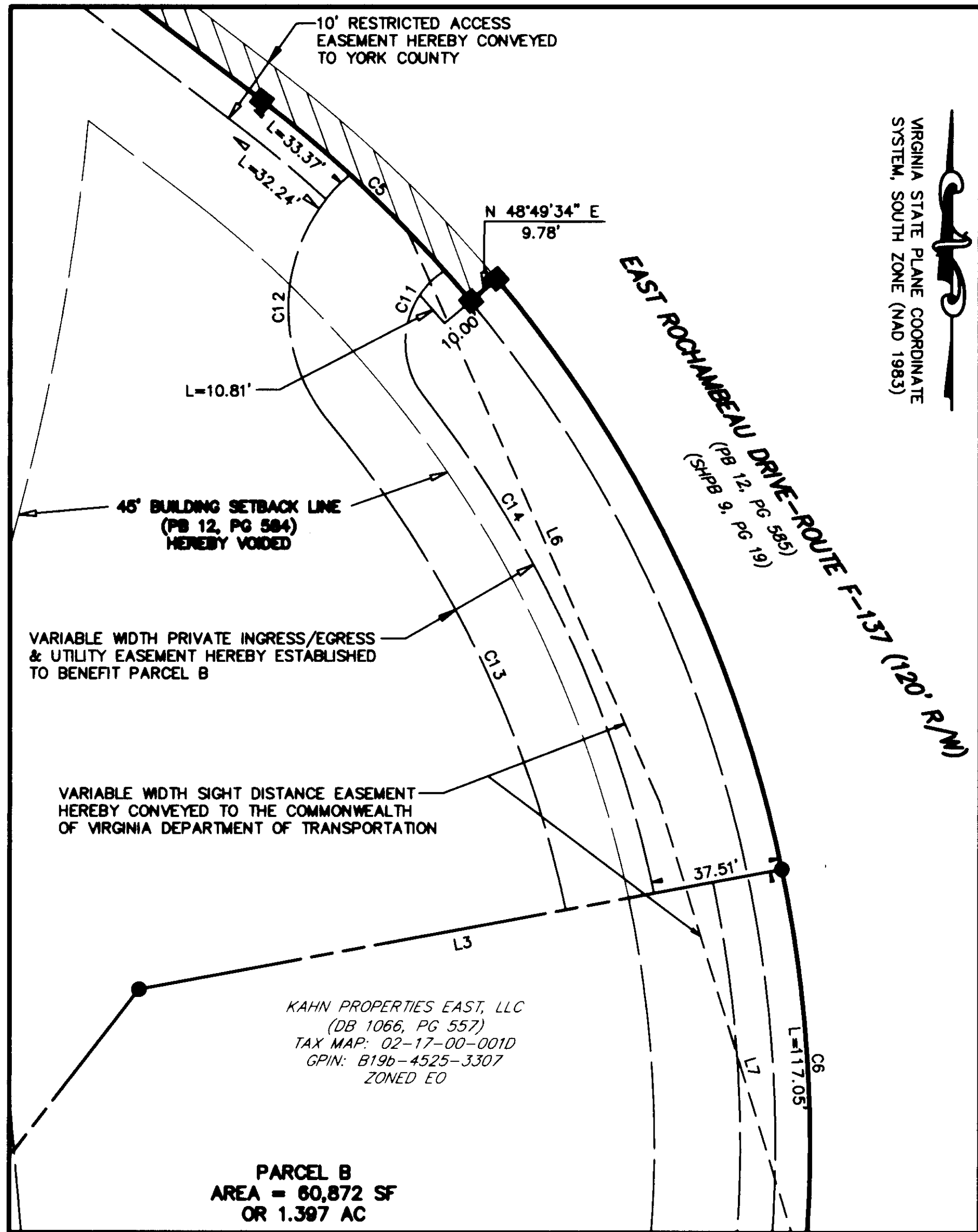
DETAIL 'A' 1"=30'
