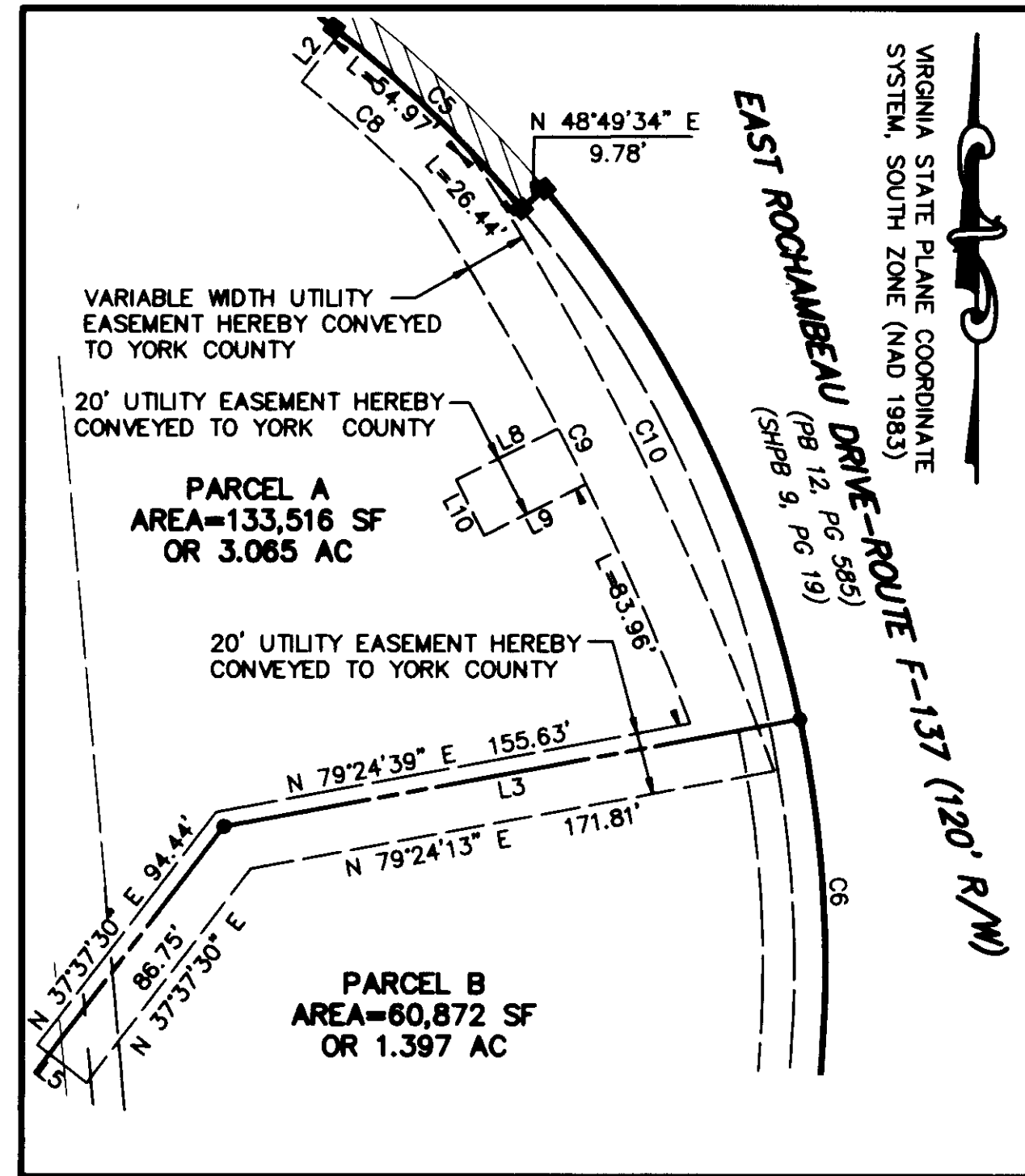
DETAIL 'B' 1"=50'
