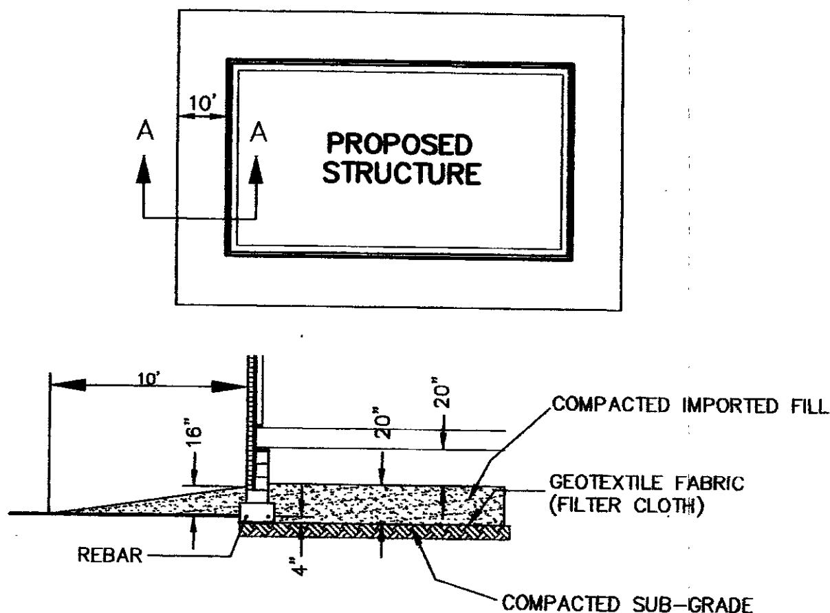
SECTION A-A MITIGATION CONSTRUCTION DETAIL
