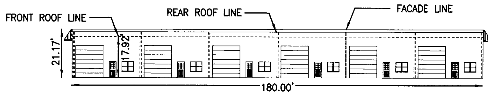
FRONT VIEW
