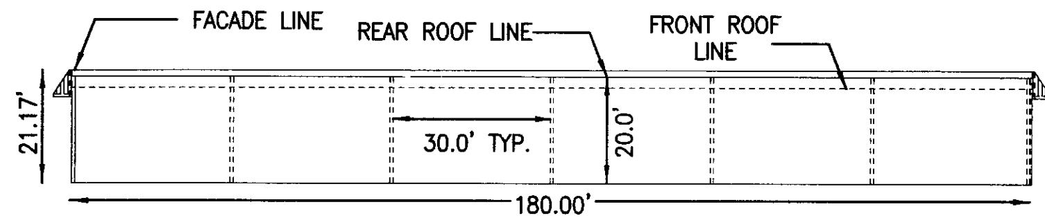
REAR VIEW
