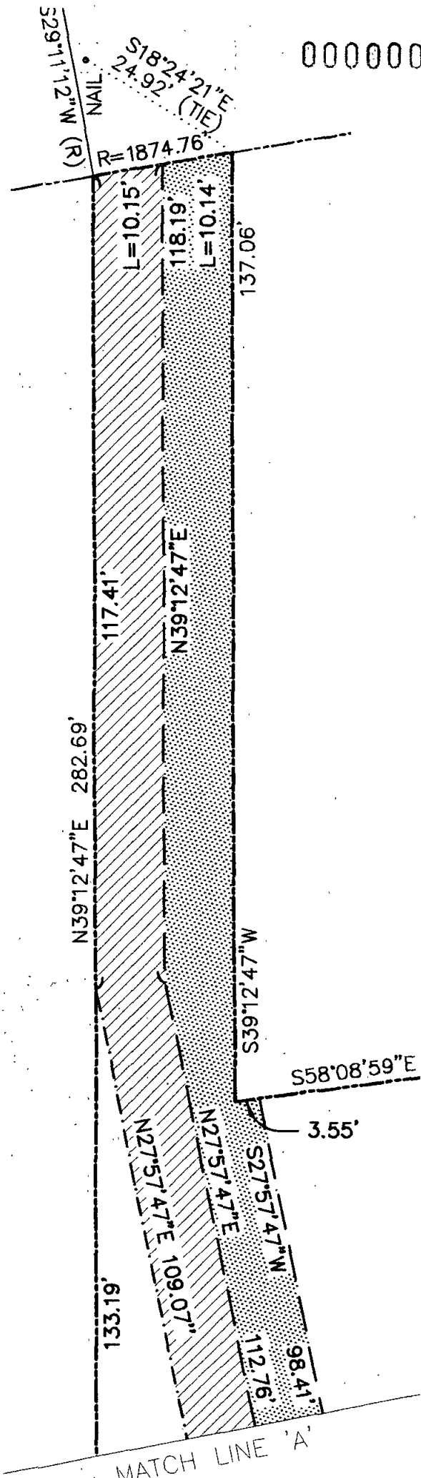
DETAIL 'A' SCALE: 1" = 20'
