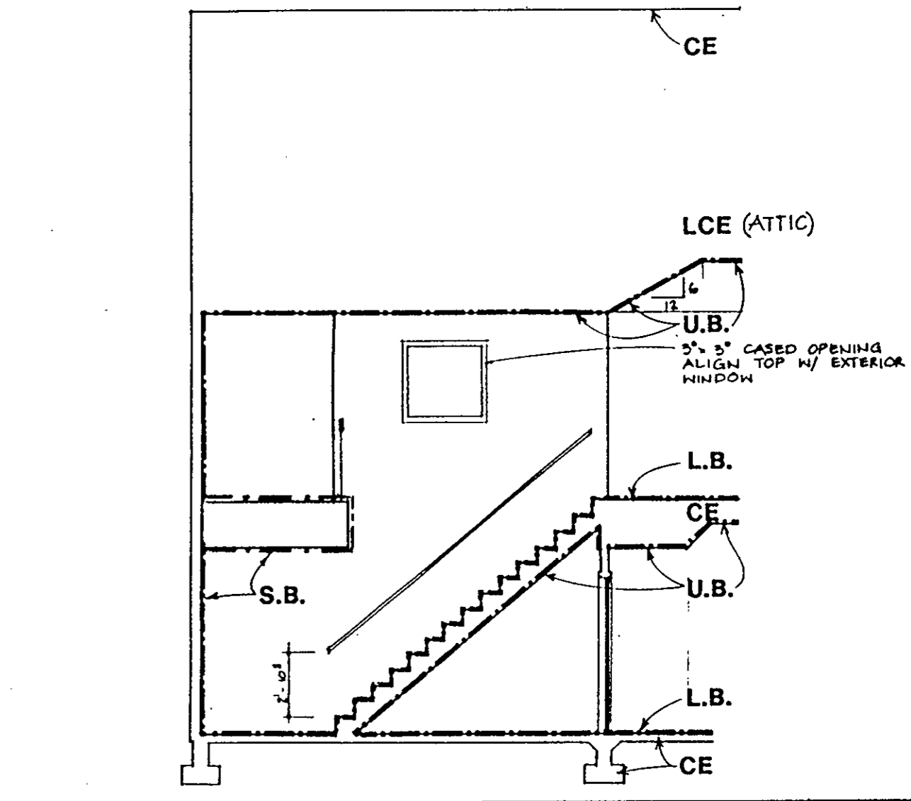
5 BUILDING SECTION THRU UNIT 'D'
