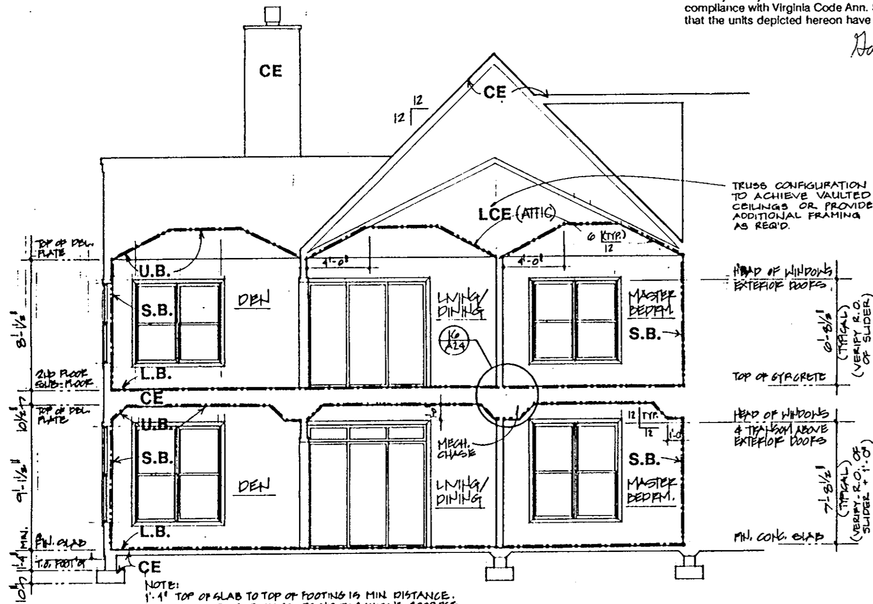
1 BUILDING SECTION THRU UNIT 'A'
