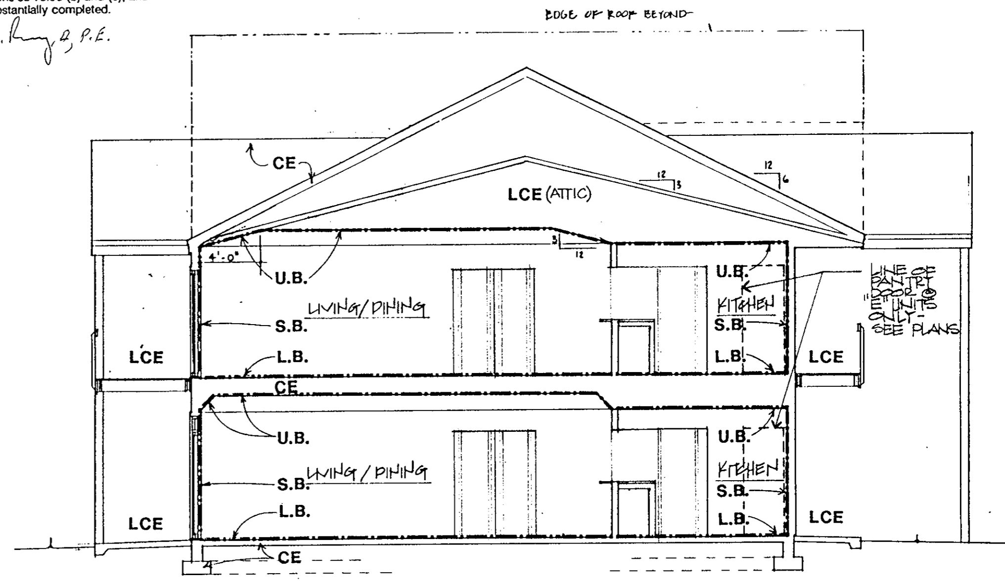
2 BUILDING SECTION THRU UNIT 'E', 'E' ALT. - SIM.
