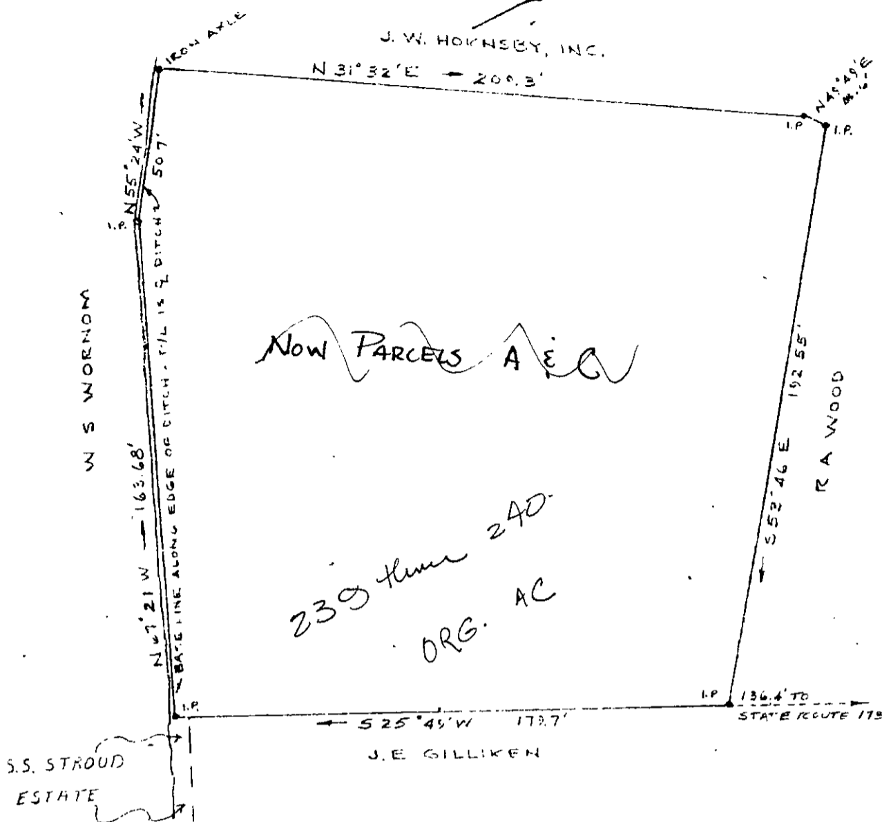
PLAT SHOWING A PARCEL OF LAND BEING PART OF THE S.S. STROUD ESTATE SITUATED IN SEAFORD, YORK COUNTY, VA. SURVEYED APRIL, 1957 SCALE 1"=40'
