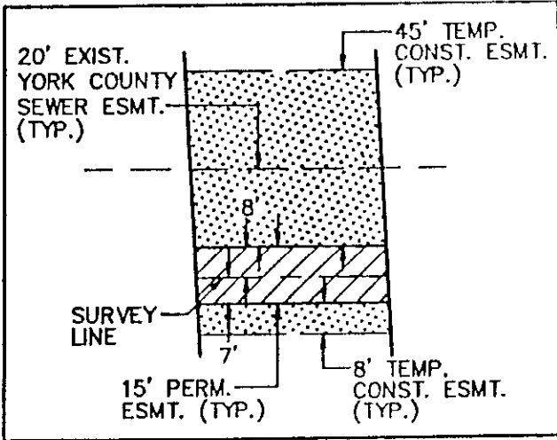
TYPICAL EASEMENT PLAN N.T.S.
