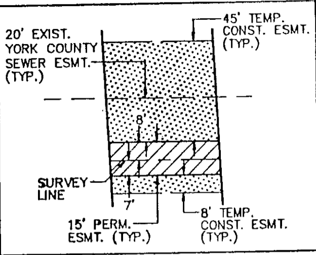
TYPICAL EASEMENT PLAN N.T.S.
