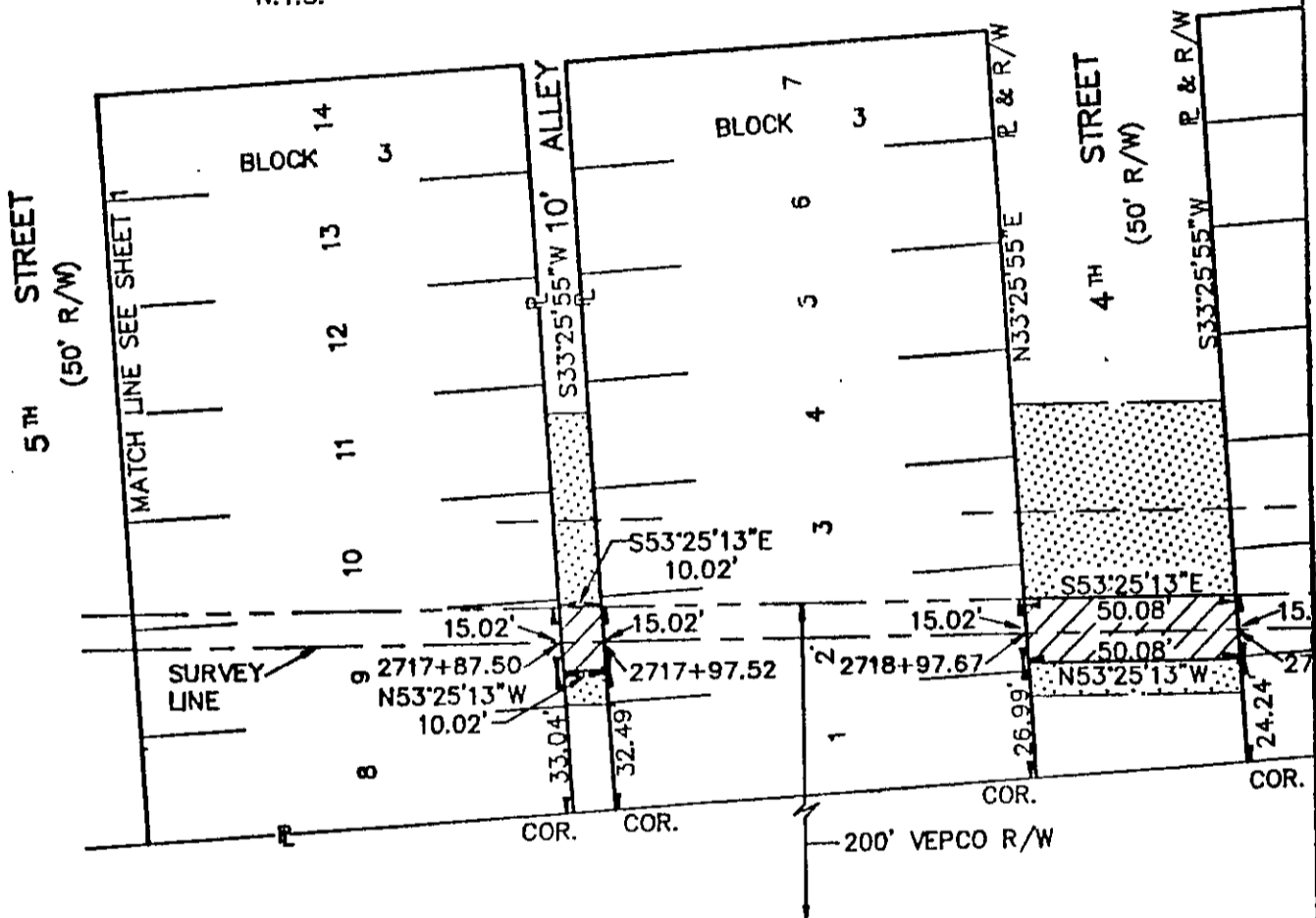
TYPICAL EASEMENT PLAN N.T.S.
