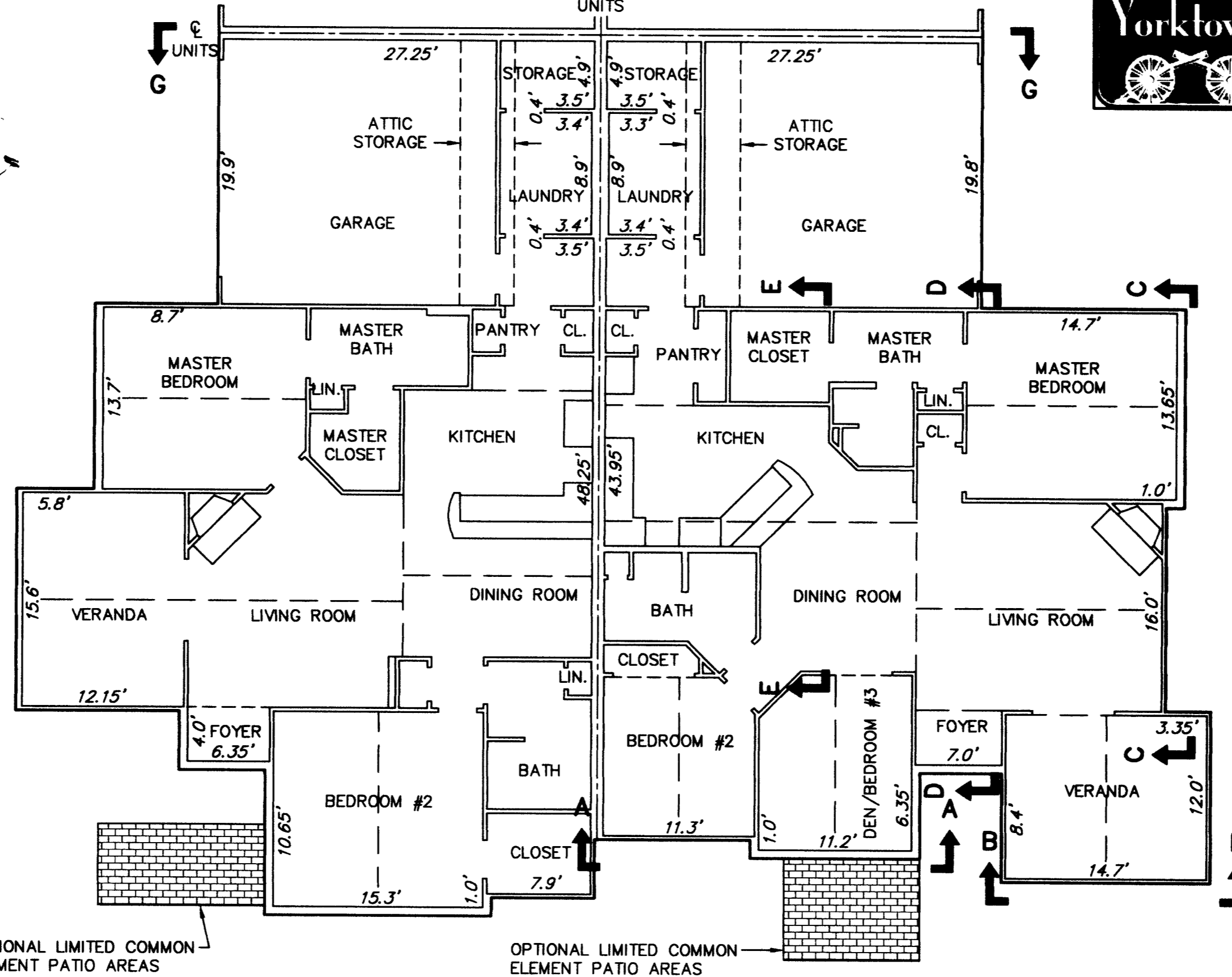
BUILDING 5-2 ABBEY FLOOR PLAN
