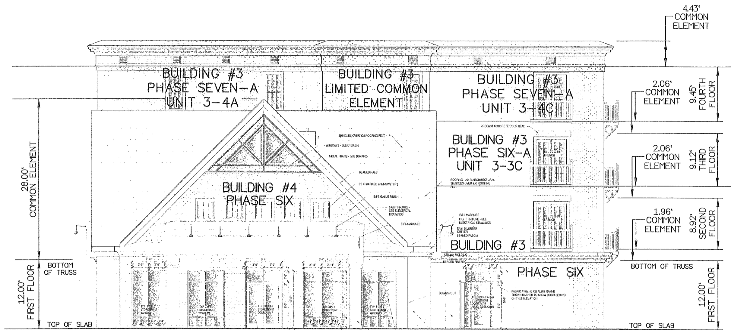
BUILDINGS #3 & #4 - RIGHT SIDE ELEVATION
