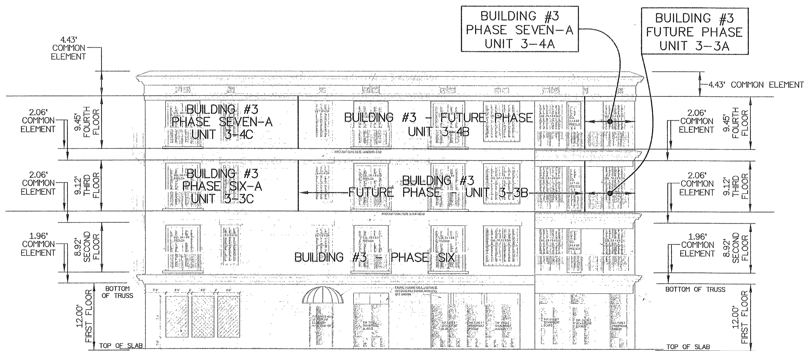
BUILDINGS #3 & #4 - LEFT SIDE ELEVATION
