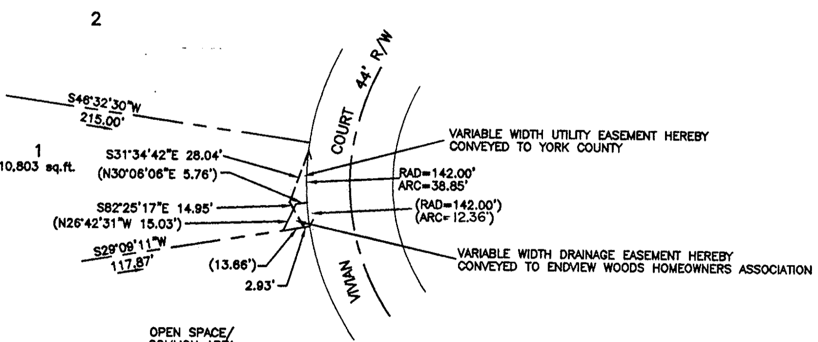
DETAIL—LOT 1 UTILITY & DRAINAGE EASEMENTS
