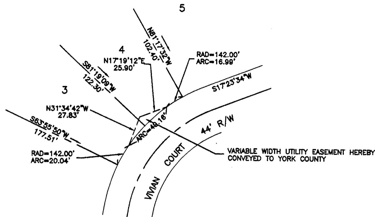
DETAIL—LOTS 3&4 UTILITY EASEMENT
