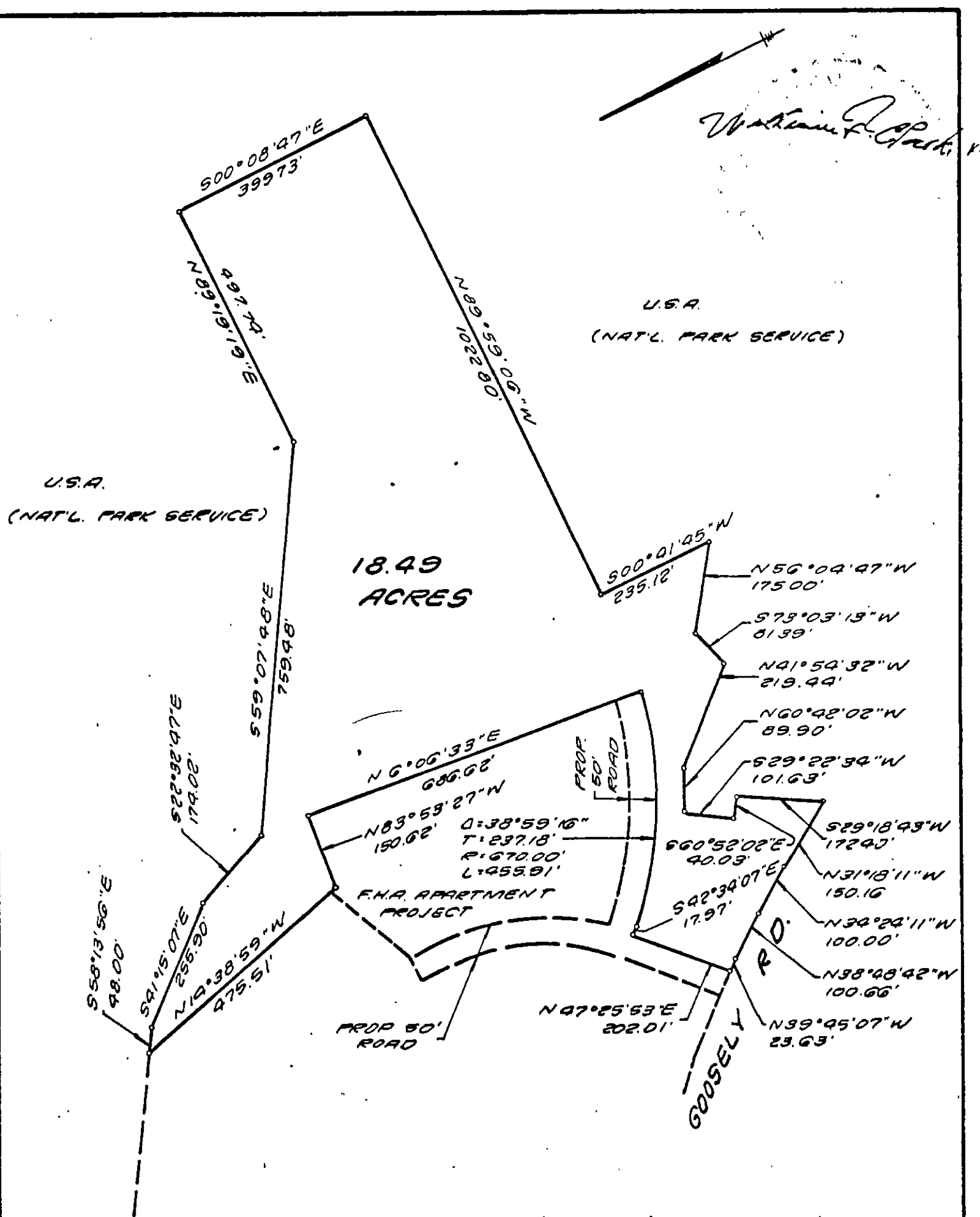
Survey and Map of Yorktown Gardens Apartment Site, Nelson District, in the County of York, Virginia.
