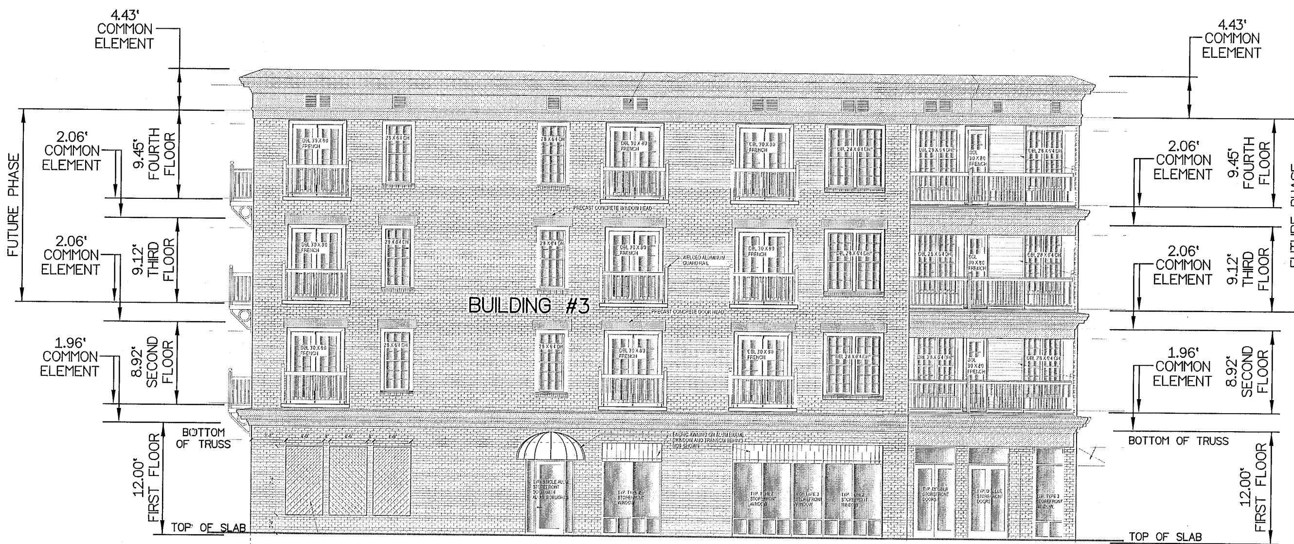
BUILDINGS #3 & #4 - LEFT SIDE ELEVATION
