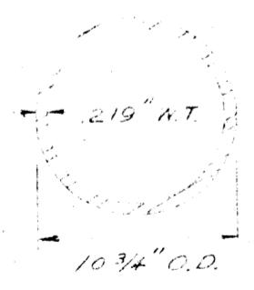
Cross Section of Steel Pipe to be installed
