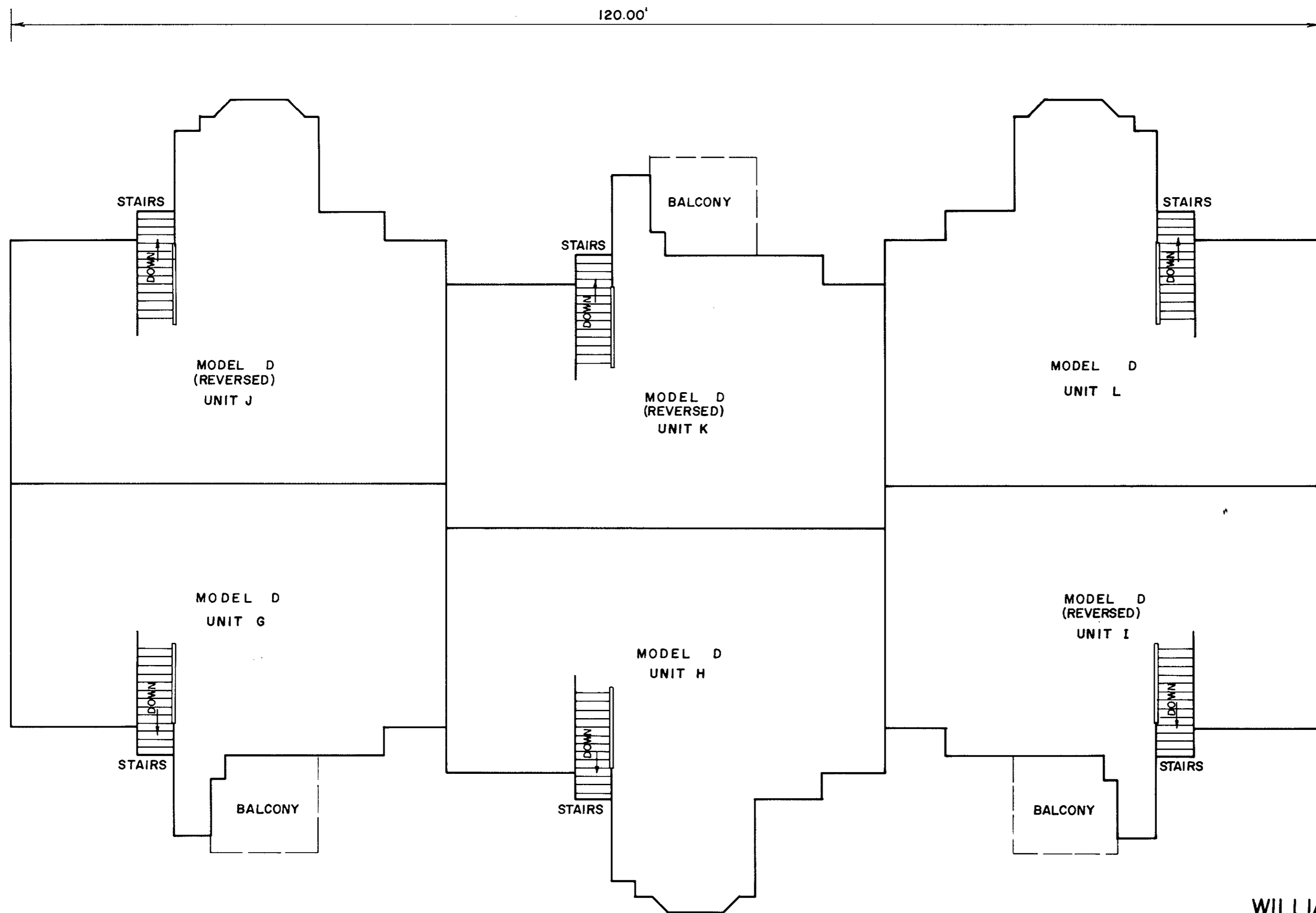
( REAR ) SECOND FLOOR BUILDING 2
