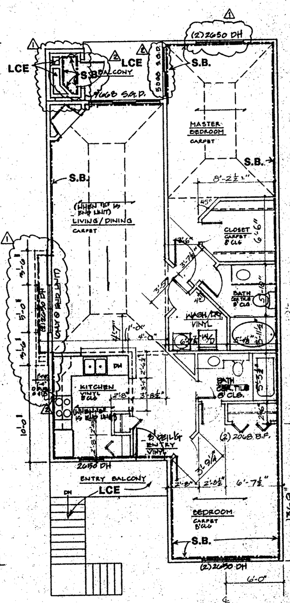
SECOND FLR. PLAN - UNIT 'E'
