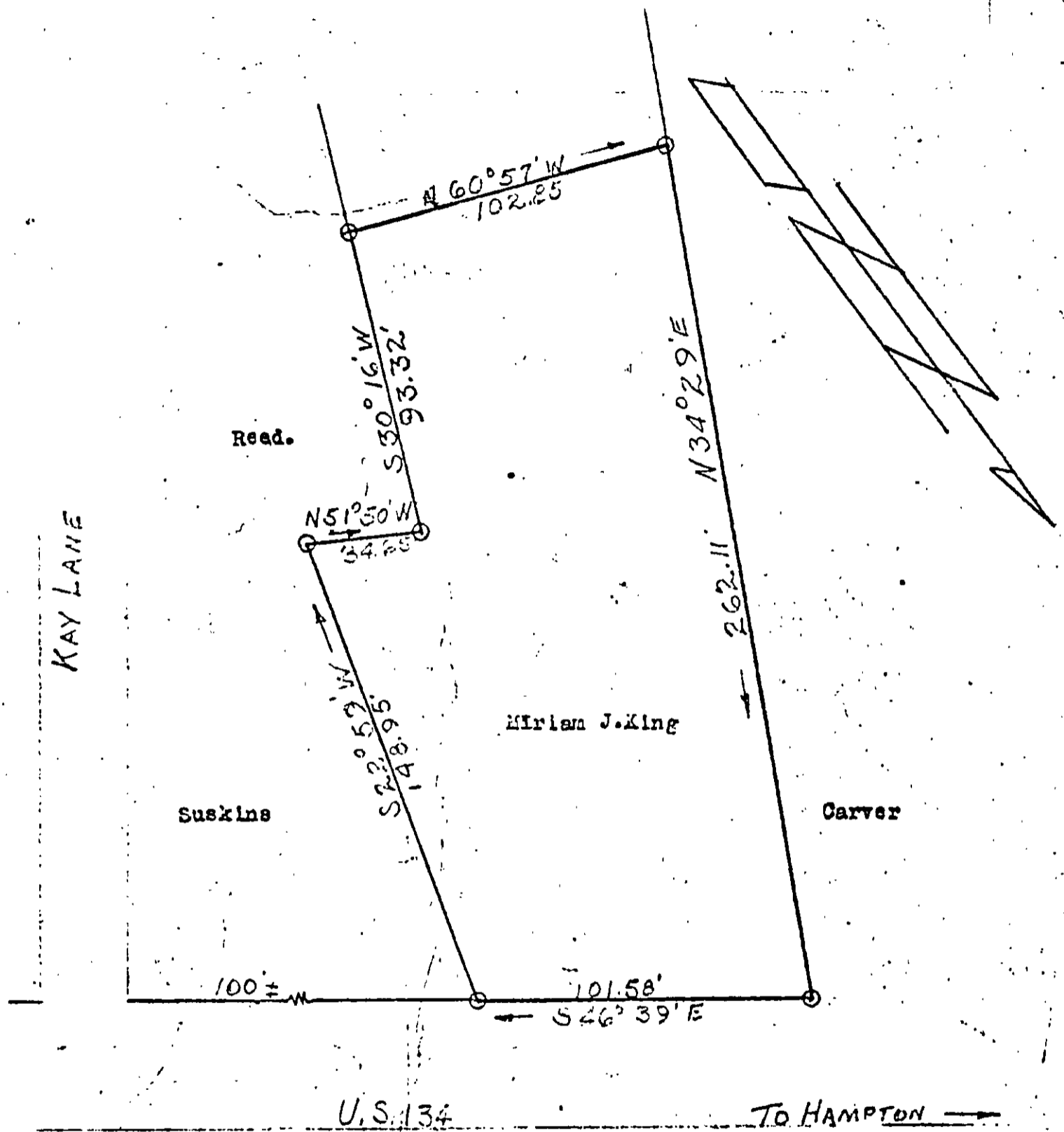
Survey showing property of Miriam J. King in Bethel Mag. Dist. York County Virginia. Ralph D. Witt Engineer Scale 1"=40' June 1966
