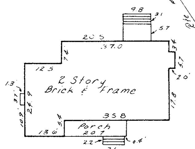
Detail of House Scale 1"=20'
